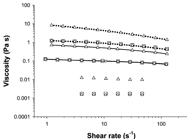
Figure 1. Viscosity curves of the nine o/w emulsions at different RO concentrations \circ = 0.5 ; \square = 3 ; \triangle = 30 g/100 g) and at different HPMC concentrations (without line = 0; solid line = 0.6; dotted line = 1.2 g/100 g).
